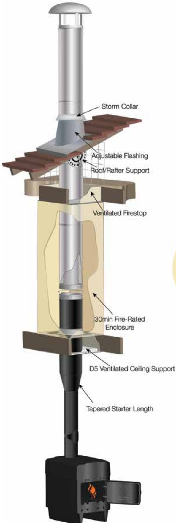
Internal System Chimney
