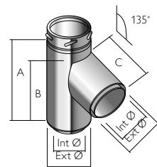
135° Tee
