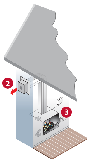
Chimney fan system with extraction via external wall – where there is no chimney
