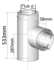
95° Reducing Tee
