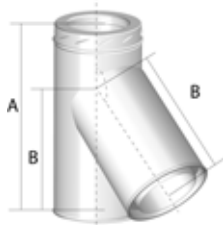
135° Tee & Elbow
