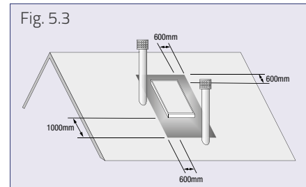
The chimney should not penetrate the dark shaded area.
