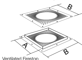
Ventilated Firestop
